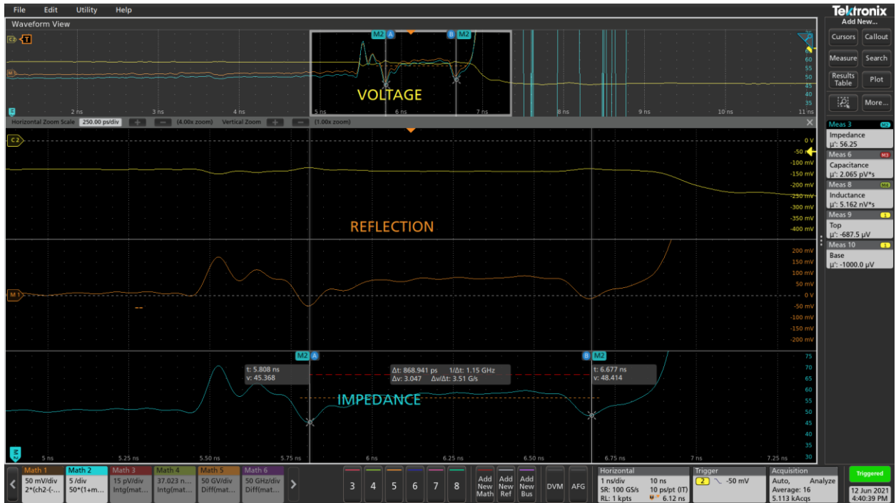
Fig. 21 - TDR Measurement of Picotest Demo Board TP5 Trace with the P2104A Probe.
