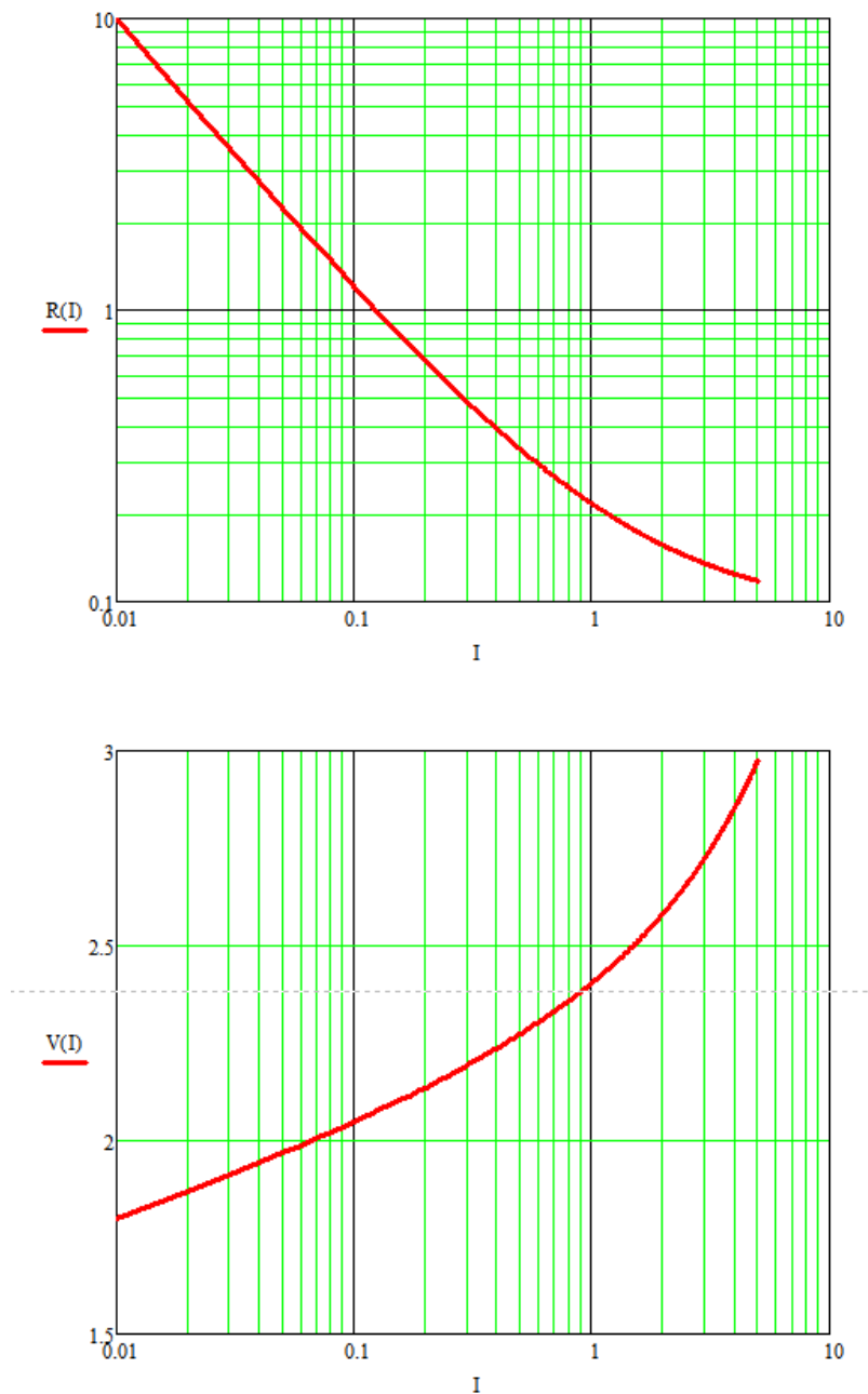
Figure 20: the voltage drop of the J2123A is graphically represented above.
