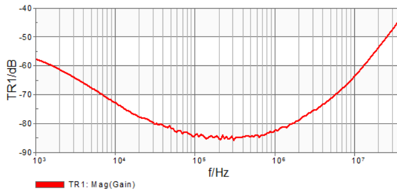
Figure 35: Common Mode Frequency response of the J2102B.
