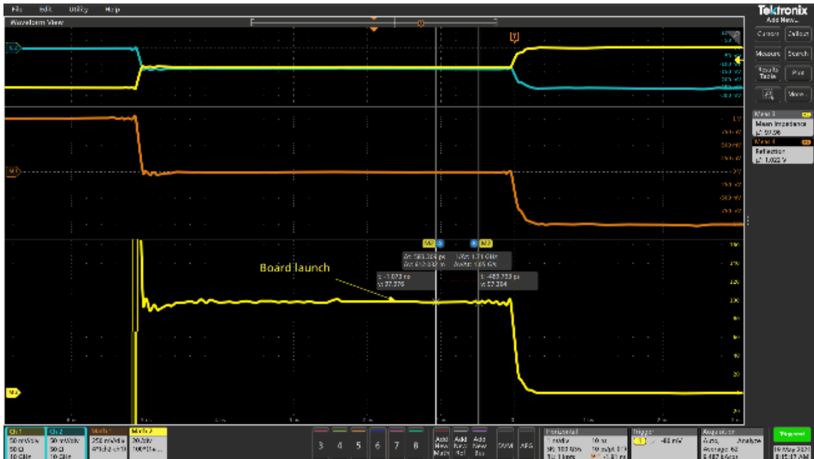
Figure 6: The P2103A recorded differential signal, gamma function and 100 Ohm measurement.
