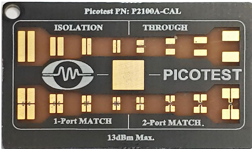
Figure 28: P2100A -CAL probe calibrator board showing the open short and load (50 Ohm) pads for different sized probe heads.
