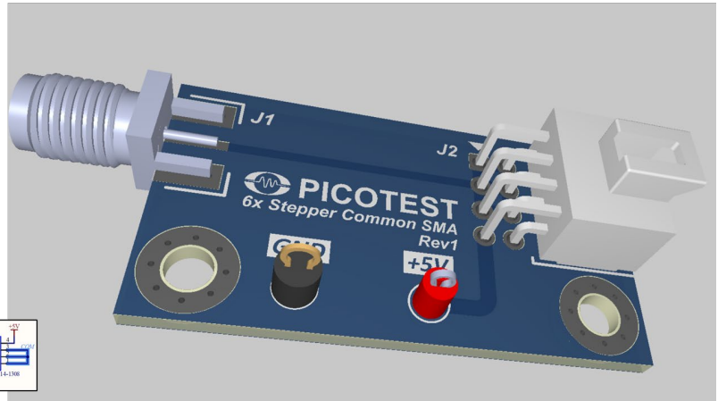
Figure 19: The S50COMMON common breakout board allow you to turn on and off all 6 switches to control a ‘full load’ current step.
