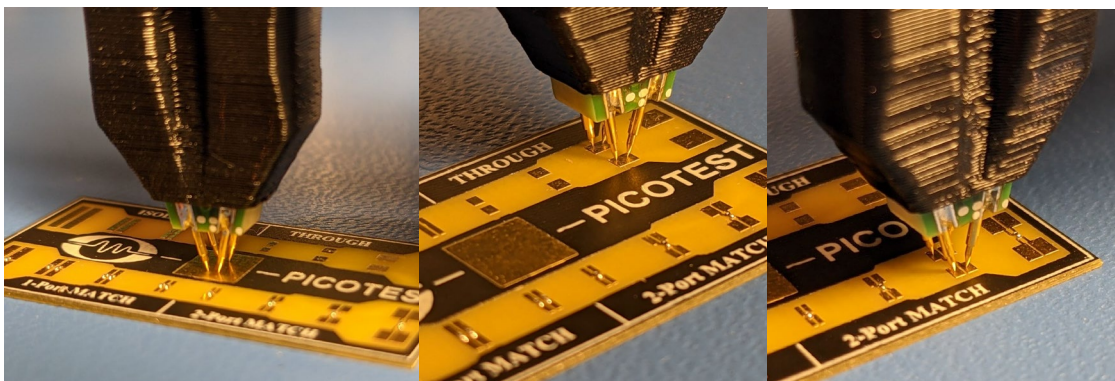
Figure 29: Performing an SOL calibration: Short (left), Open (center), and load (50 Ohm, right) calibration.
