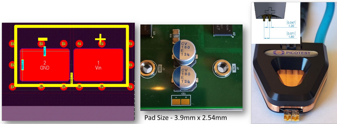
Figure 16: Suggested solder pad size.
