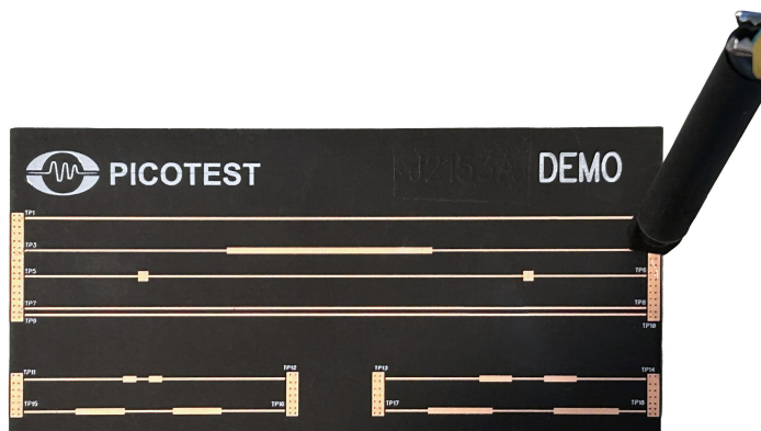
Making a TDR measurement on a PCB trace with impedance variations. Note how the trace widens in the center.
